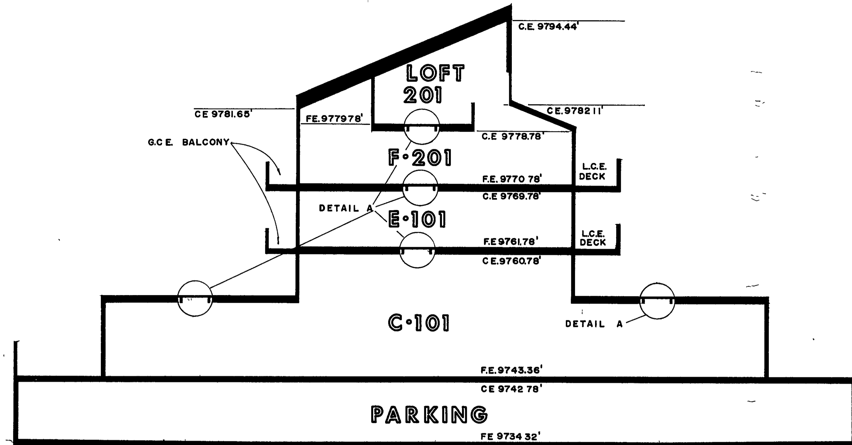
SECTION E-E
