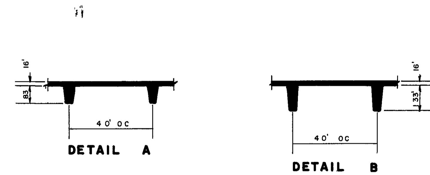
STRUCTURAL 'T' DETAIL
